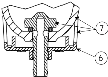
SECTION VIEW (Plastic Bowl Manual Drain)
