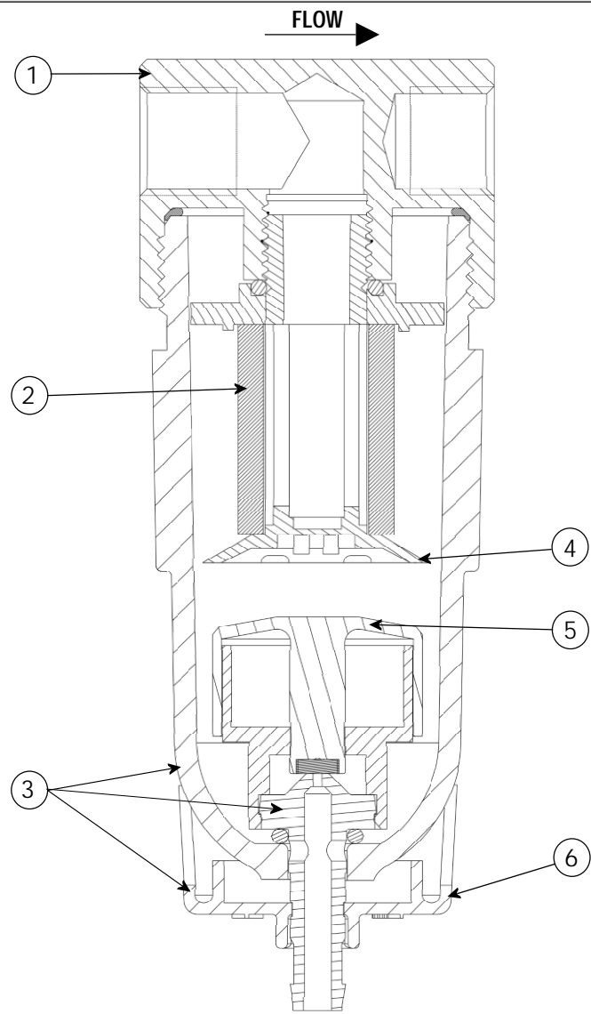
FD50 SECTION VIEW (Plastic Bowl Automatic Internal Drain)
